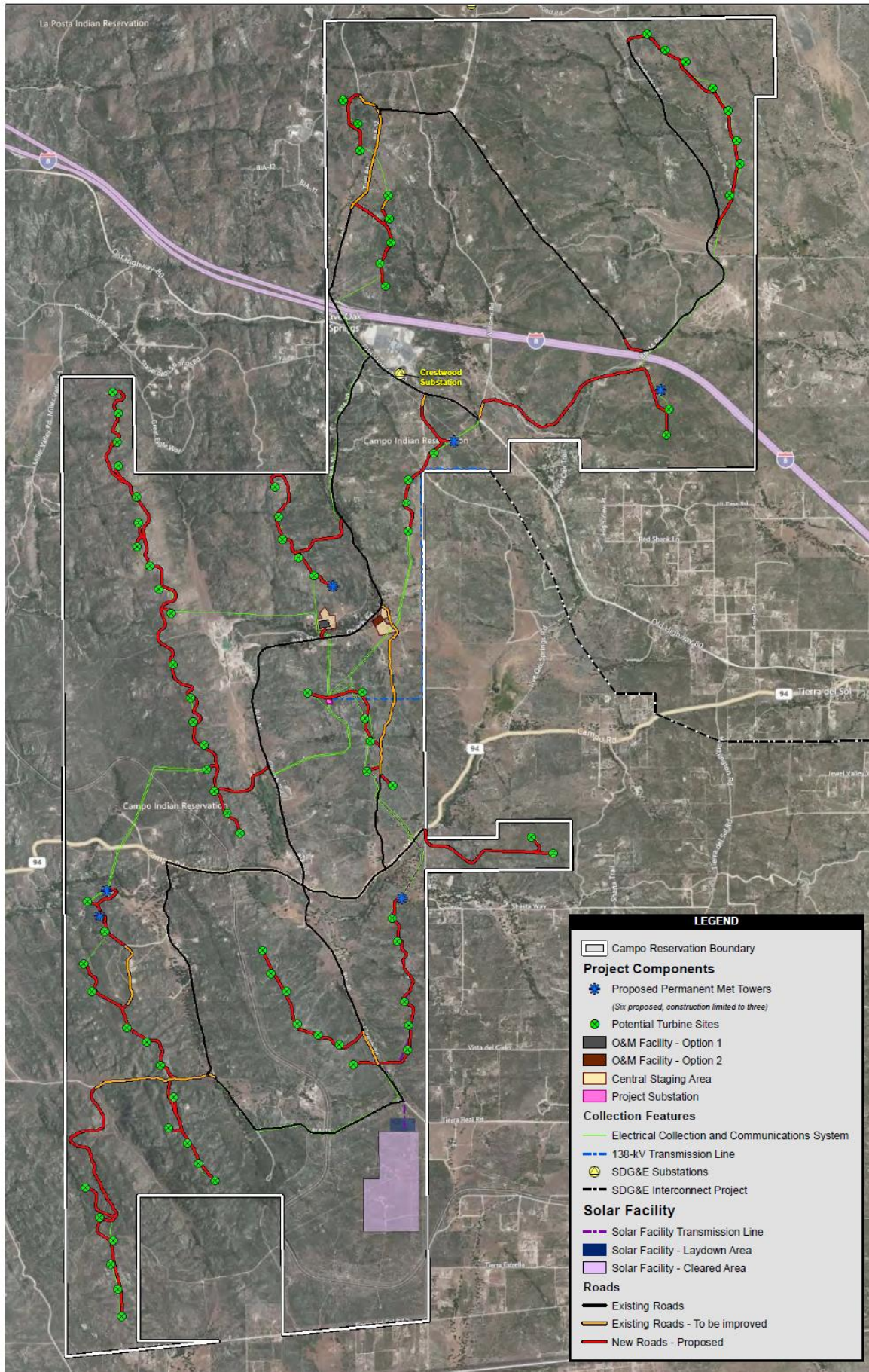
Figure 2-9 Working Design Project Components - Alternative 1
