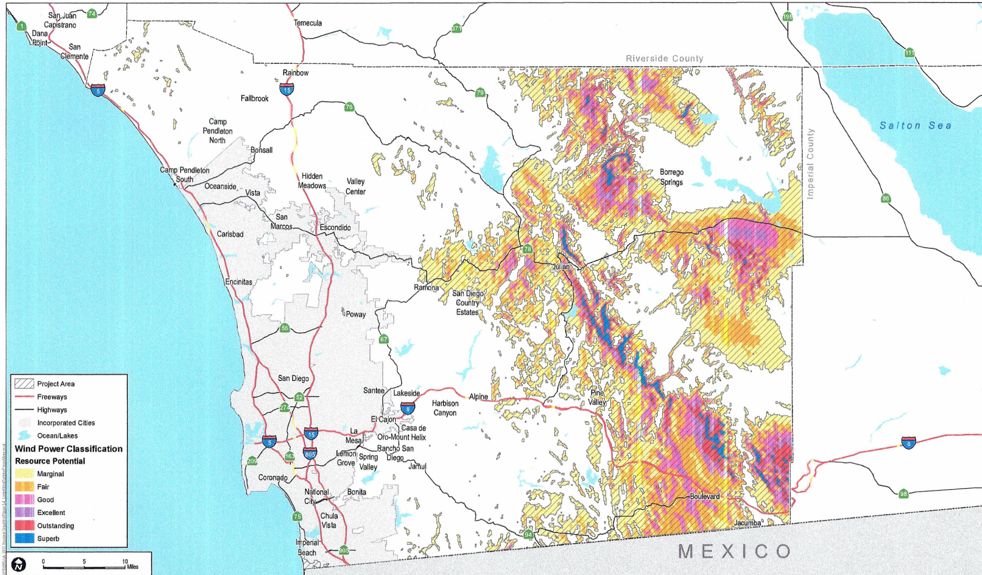
FIGURE 1-4 Large Wind Turbine(s) Project Area
